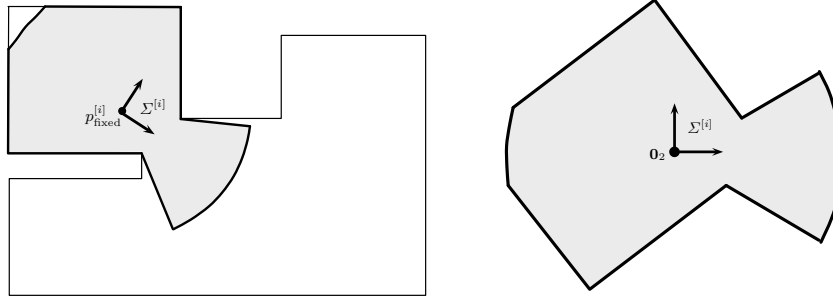
Figure 3.8 The left-hand plot depicts the range-limited visibility set \text{Vi}_{\text{disk}}(p_{\text{fixed}}^{[i]}; Q) expressed with respect to an inertially fixed frame. The right-hand plot depicts the range-limited visibility set expressed with respect to the body-fixed frame \Sigma^{[i]} , that is, \text{Vi}_{\text{disk}}(\mathbf{0}_2; Q_i) .
