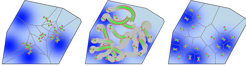
Figure 5.3 The evolution of (\mathcal{S}_D, \text{VRN-CNTRD-DYNMCS}) with n = 20 robots and with feedback gain k_{\text{prop}} = 3.5 . The left-hand (resp., right-hand) figure illustrates the initial (resp., final) locations and Voronoi partition. The central figure illustrates the evolution of the robots. After 20 seconds, the value of \mathcal{H}_{\text{dist}} has monotonically increased to approximately -0.555 .
