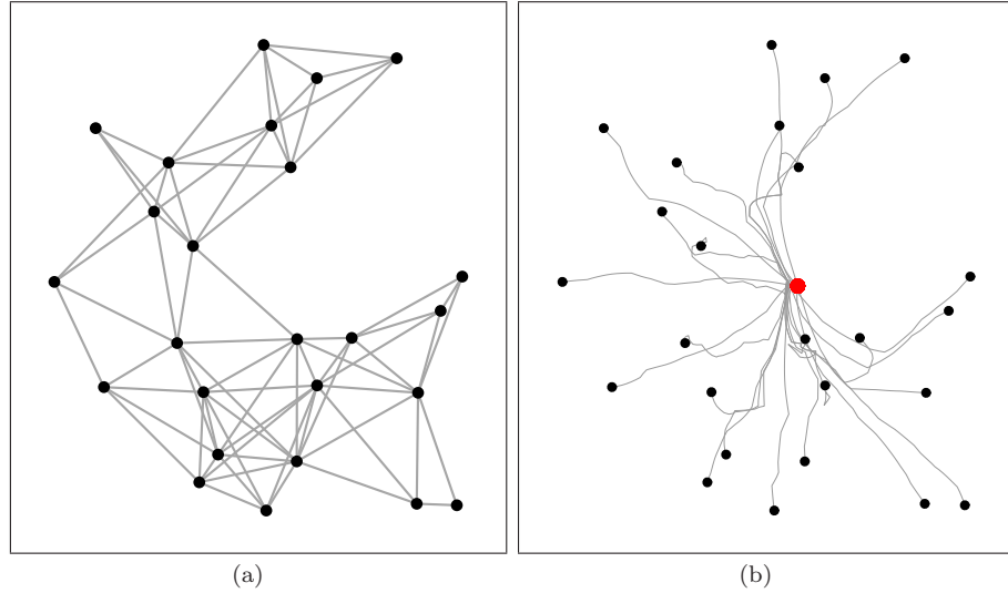
Figure 4.11 The evolution of (\mathcal{S}_{\infty\text{-disk}}, \text{PLL-CRCMCNTR}) with n = 25 robots in 2 dimensions: (a) shows the initial connected network configuration; (b) shows the evolution of the individual agents until rendezvous is achieved.
